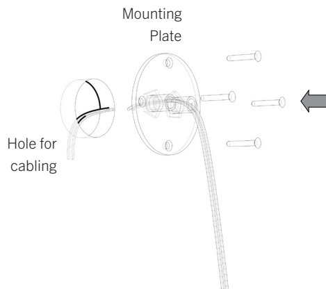
5 Low Voltage Electrical Connection
