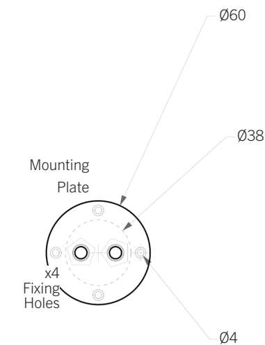
3 Mounting Orientation
