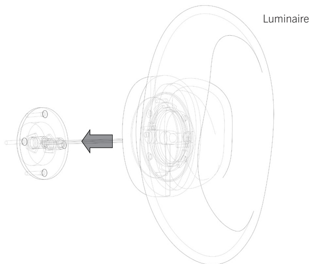
7 Slide On Luminaire
