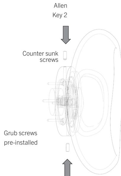
8 Lock Luminaire In Place
